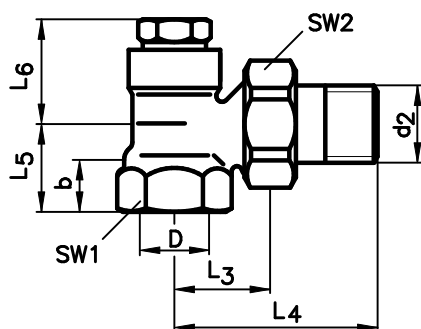
Type 456 S, M – angled, version BG
