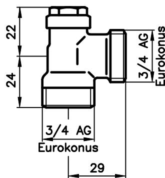
Type 456 S, M – angled, version BG
