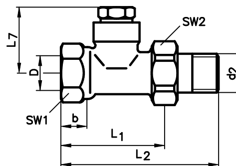
Type 456 S, M – straight, version BG
