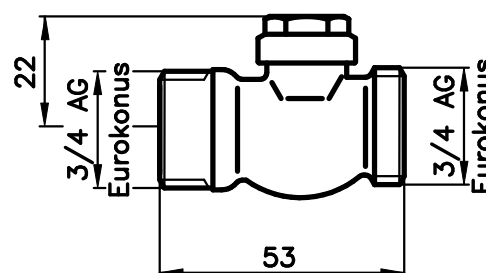
Type 456 S, M – straight, version BG
